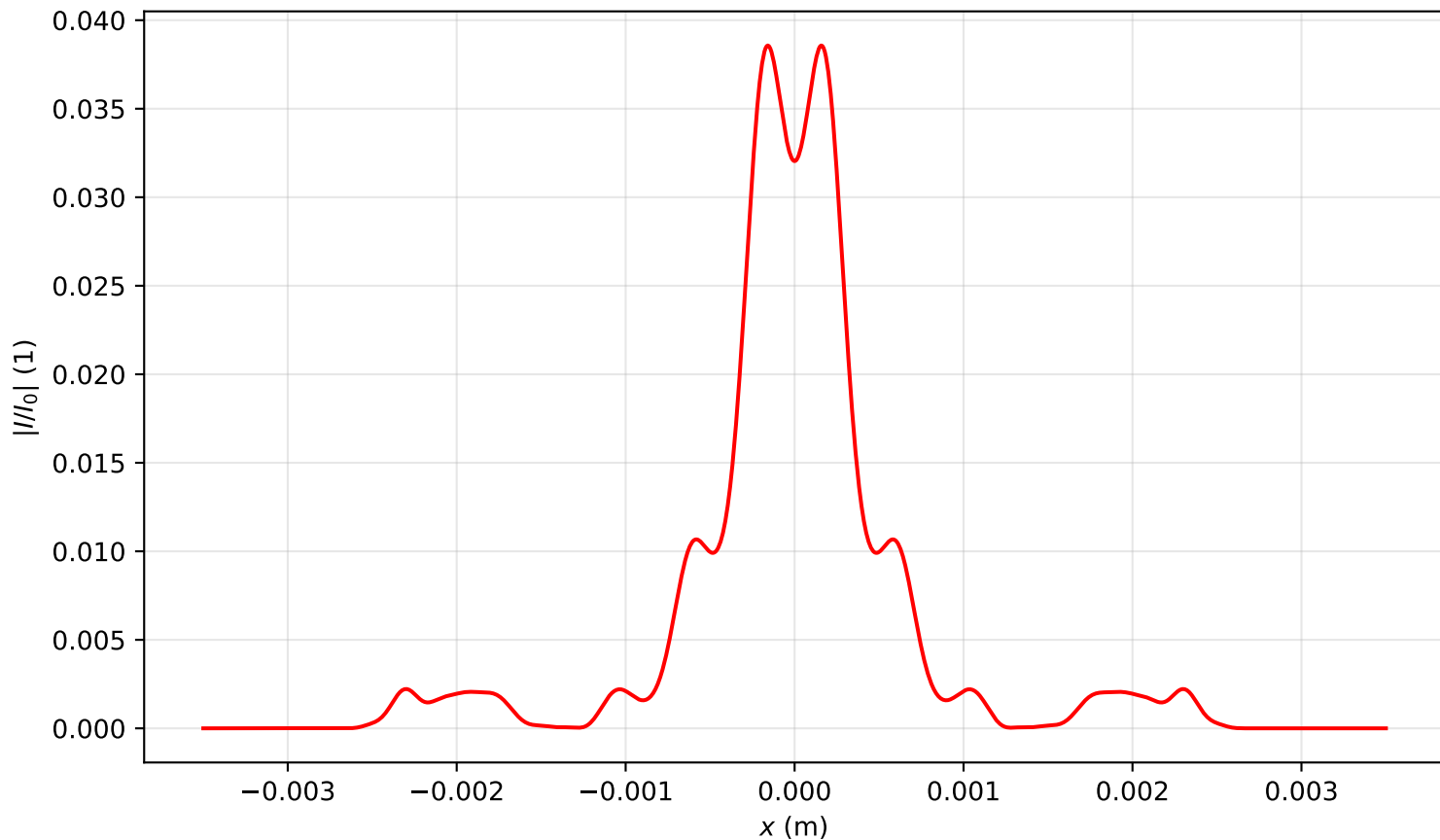
Intensity profile I(x, y = 0, z = 2.866)/I_0 , P_{in}=18.0\text{Pcr} , artificial time
