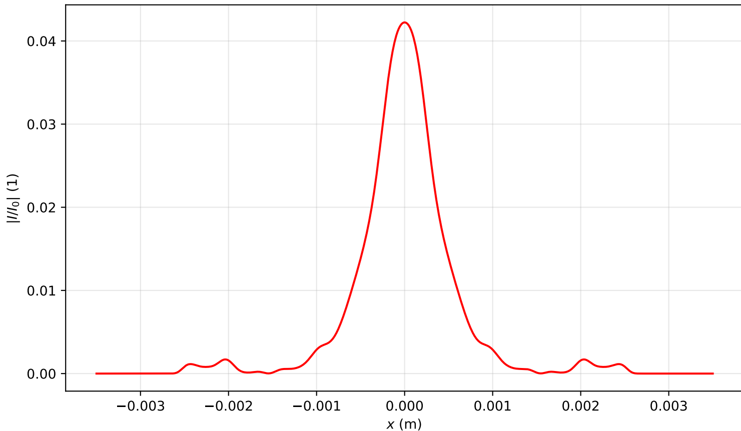
Intensity profile I(x, y = 0, z = 3.025)/I_0 , P_{in}=18.0\text{Pcr} , artificial time
