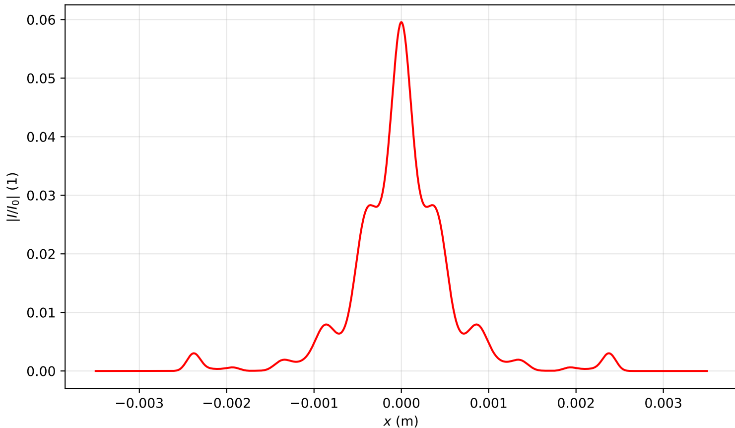
Intensity profile I(x, y = 0, z = 3.184)/I_0 , P_{in}=18.0\text{Pcr} , artificial time
