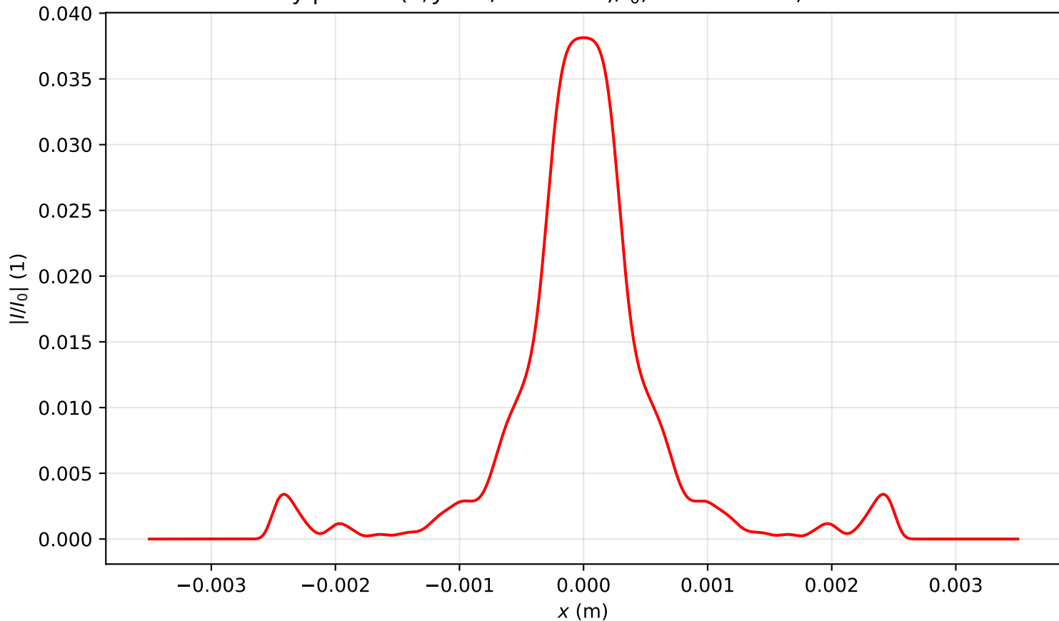
Intensity profile I(x, y = 0, z = 3.344)/I_0 , P_{in}=18.0P_{cr} , artificial time
