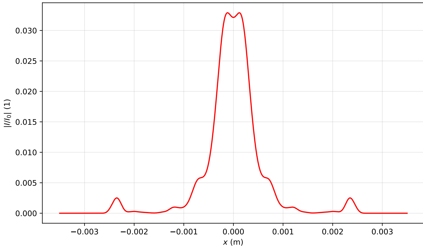
Intensity profile I(x, y = 0, z = 3.503)/I_0 , P_{in}=18.0\text{Pcr} , artificial time
