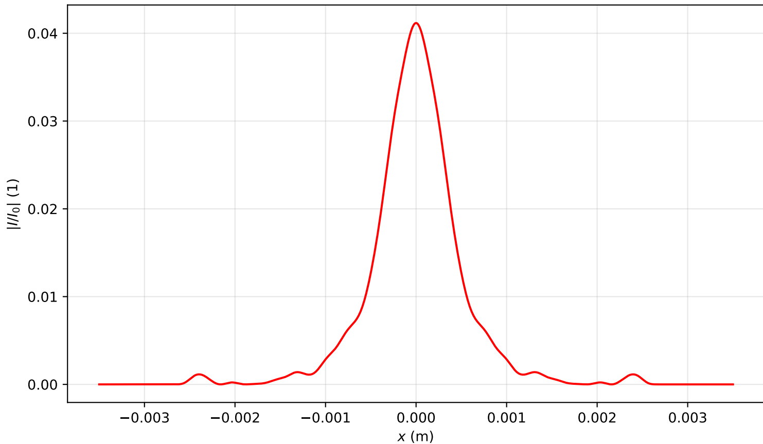
Intensity profile I(x, y = 0, z = 3.662)/I_0 , P_{in}=18.0\text{Pcr} , artificial time
