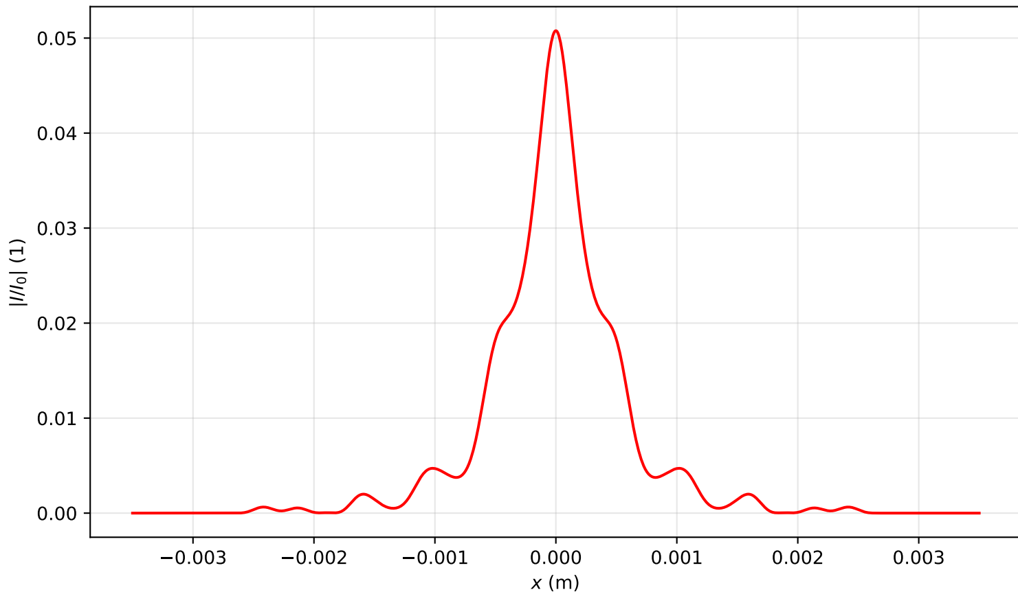
Intensity profile I(x, y = 0, z = 3.821)/I_0 , P_{in}=18.0P_{cr} , artificial time
