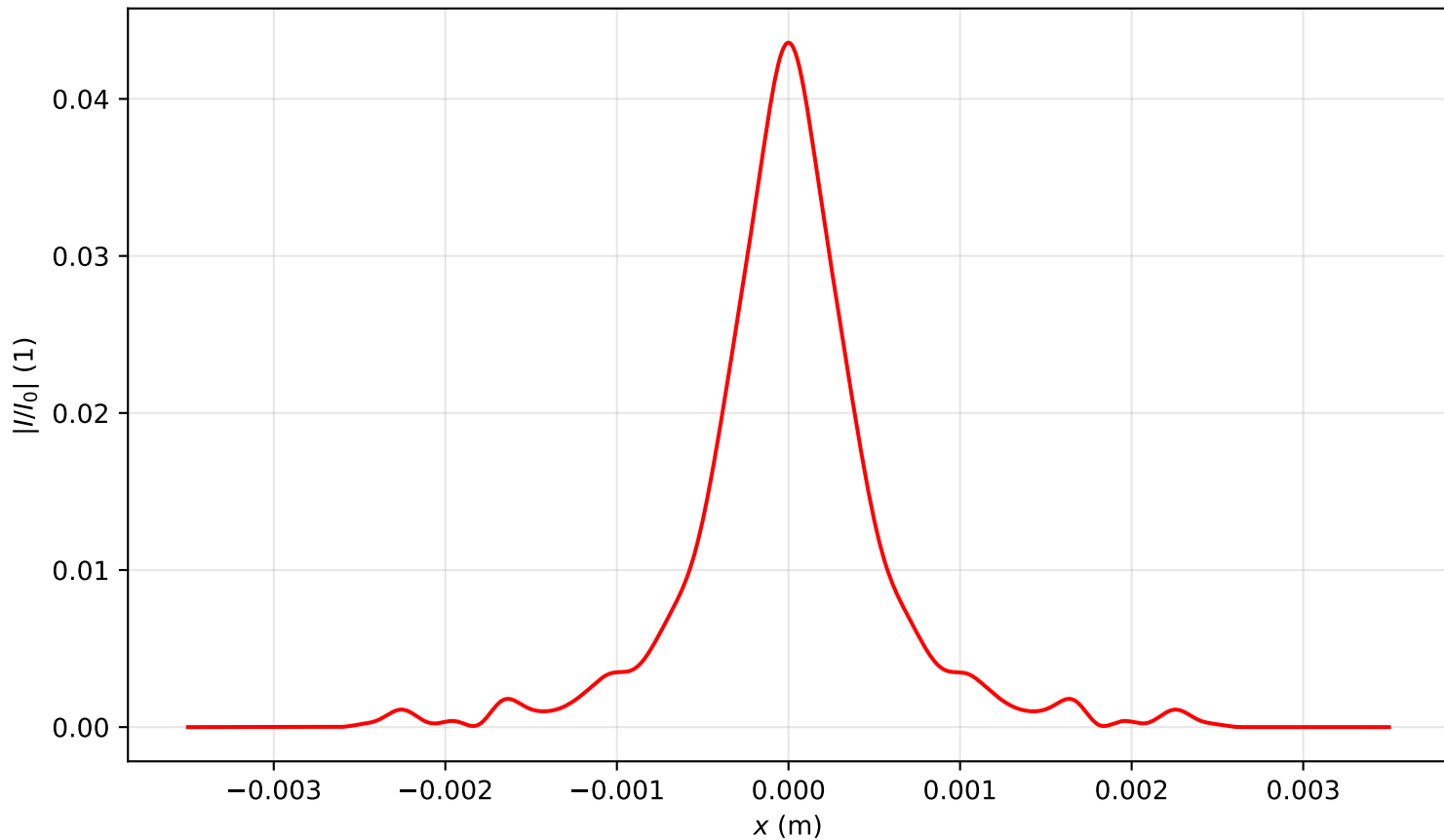
Intensity profile I(x, y = 0, z = 3.981)/I_0 , P_{in}=18.0\text{Pcr} , artificial time
