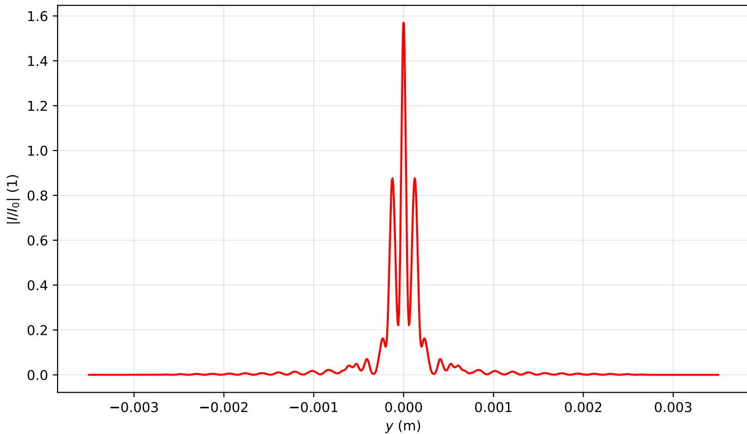
Intensity profile I(x=0, y, z=0.159)/I_0 , P_{in}=18.0P_{cr} , artificial time
