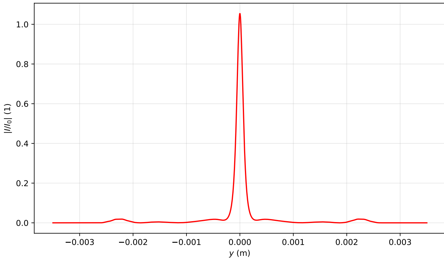
Intensity profile I(x=0, y, z=0.955)/I_0 , P_{in}=18.0P_{cr} , artificial time
