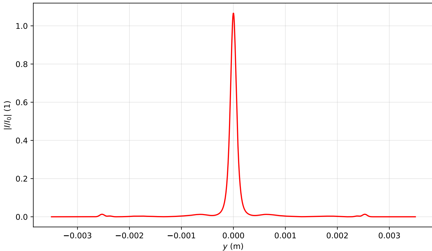
Intensity profile I(x=0, y, z=1.115)/I_0 , P_{in}=18.0P_{cr} , artificial time
