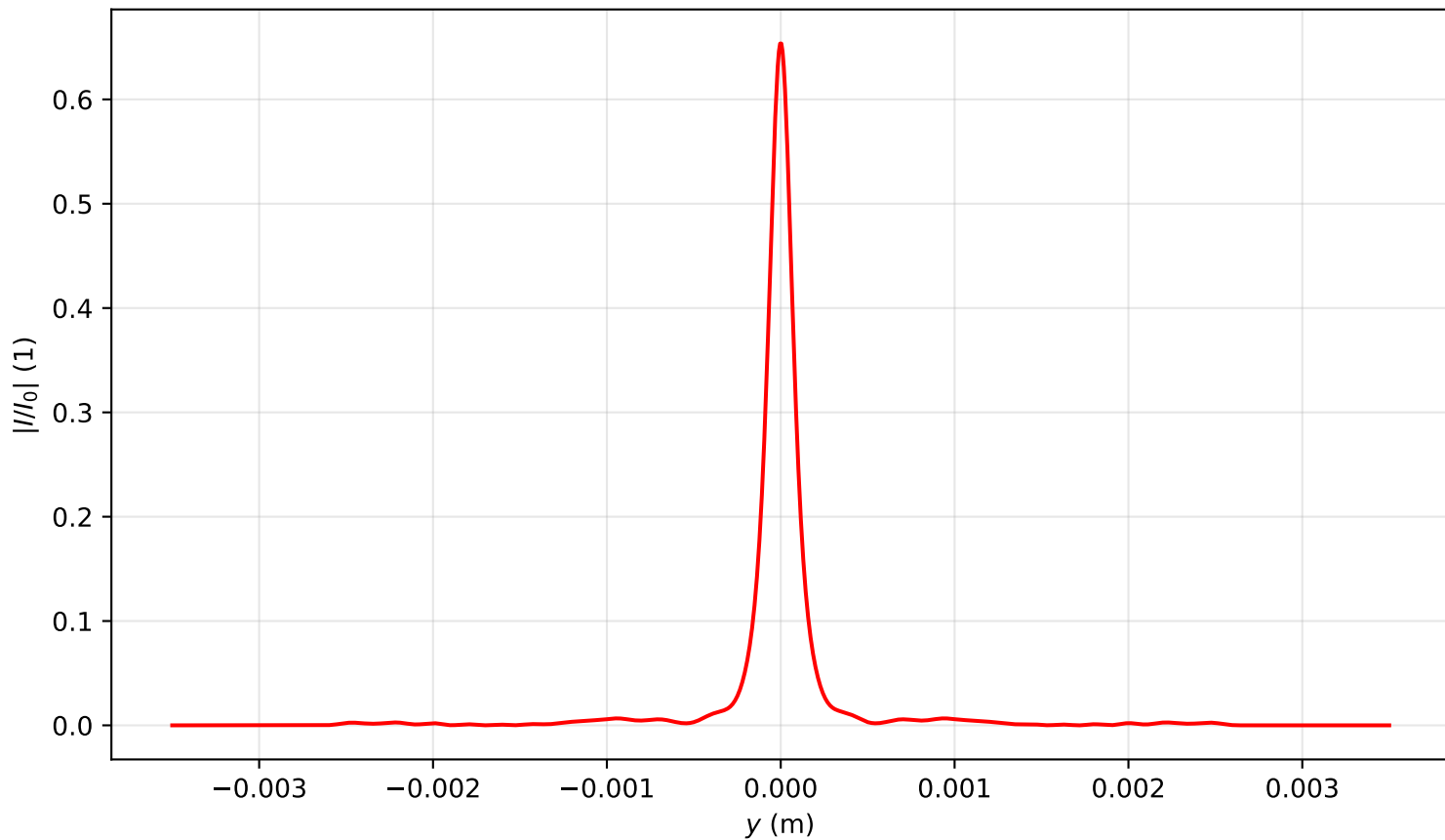
Intensity profile I(x=0, y, z=1.433)/I_0 , P_{in}=18.0P_{cr} , artificial time
