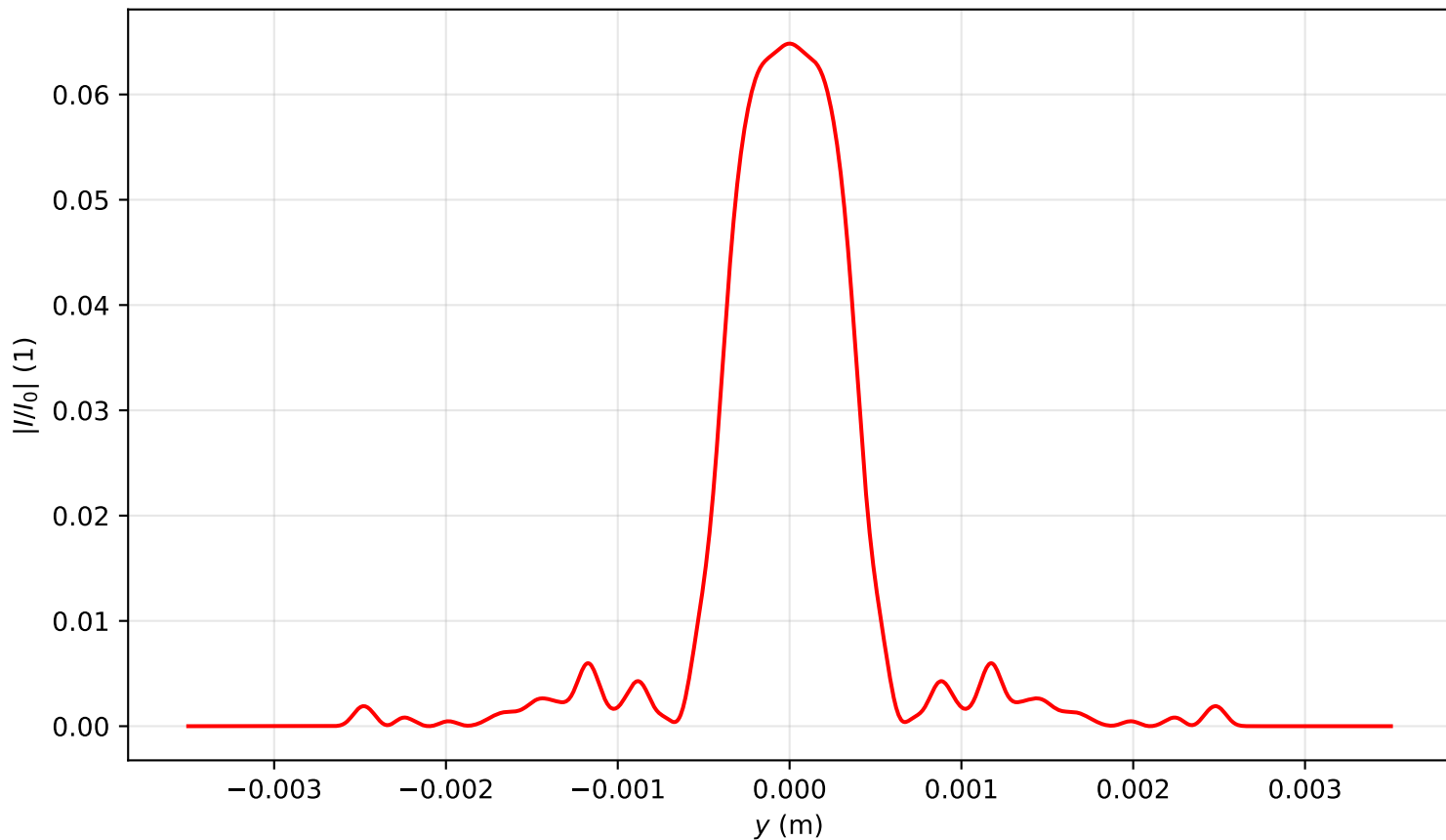
Intensity profile I(x = 0, y, z = 1.751)/I_0 , P_{in}=18.0P_{cr} , artificial time
