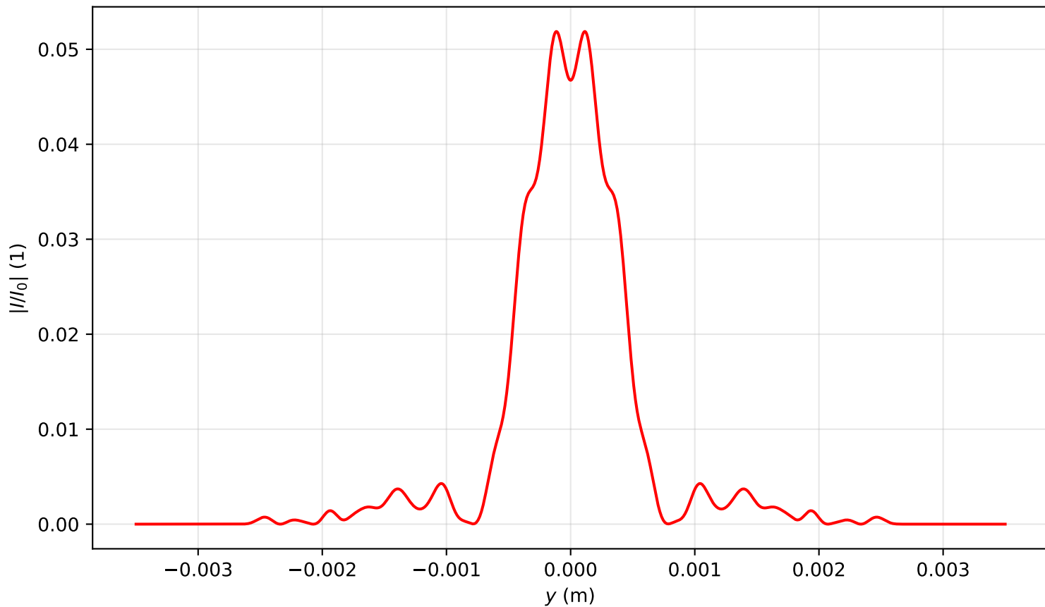
Intensity profile I(x = 0, y, z = 1.911)/I_0 , P_{in}=18.0P_{cr} , artificial time
