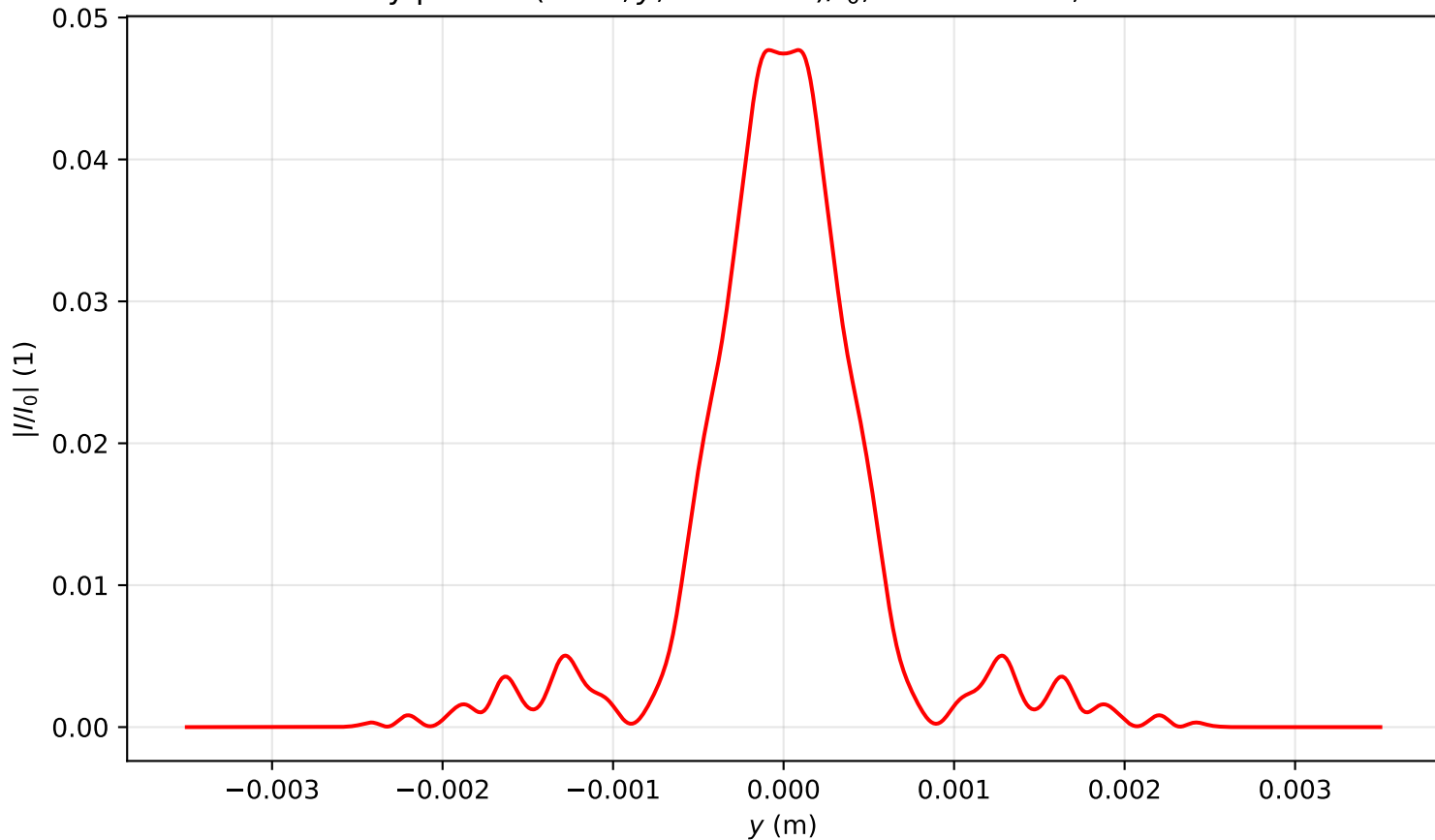
Intensity profile I(x = 0, y, z = 2.070)/I_0 , P_{in}=18.0\text{Pcr} , artificial time
