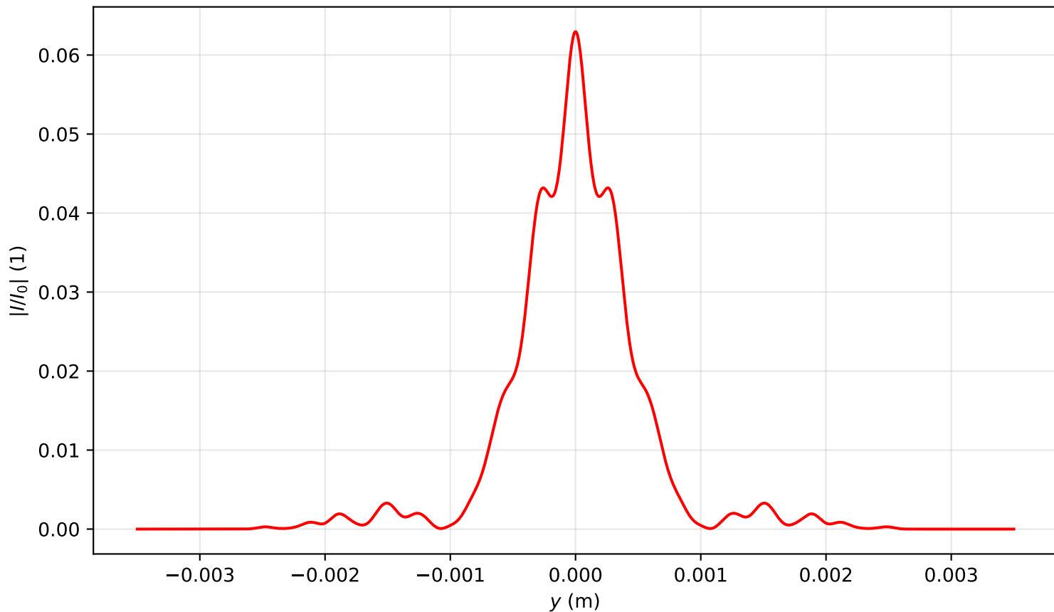
Intensity profile I(x=0, y, z=2.229)/I_0 , P_{in}=18.0P_{cr} , artificial time
