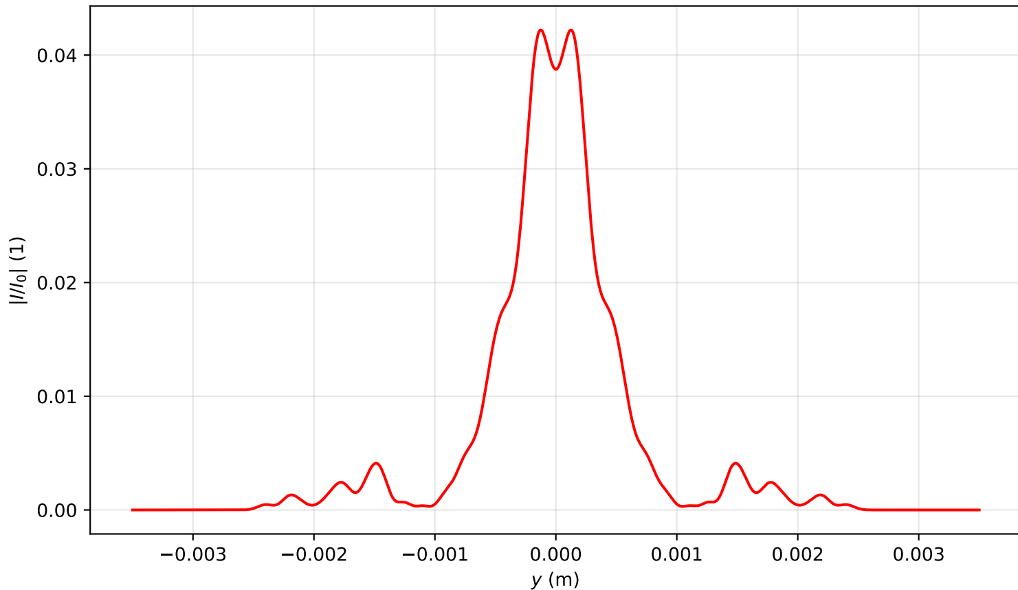
Intensity profile I(x = 0, y, z = 2.388)/I_0 , P_{in}=18.0\text{Pcr} , artificial time
