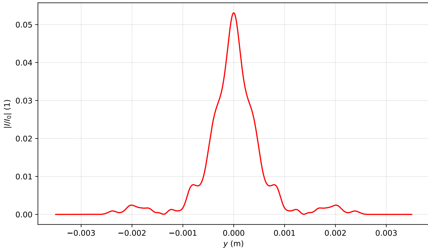
Intensity profile I(x = 0, y, z = 2.707)/I_0 , P_{in}=18.0\text{Pcr} , artificial time
