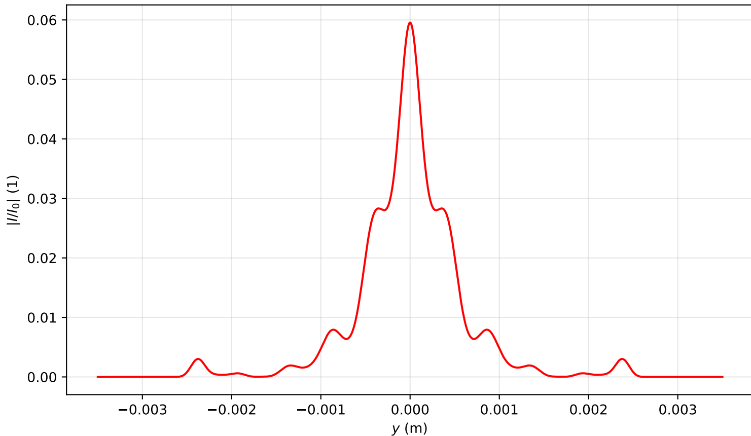
Intensity profile I(x = 0, y, z = 3.184)/I_0 , P_{in}=18.0\text{Pcr} , artificial time
