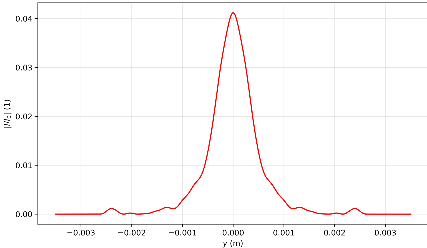
Intensity profile I(x = 0, y, z = 3.662)/I_0 , P_{in}=18.0\text{Pcr} , artificial time
