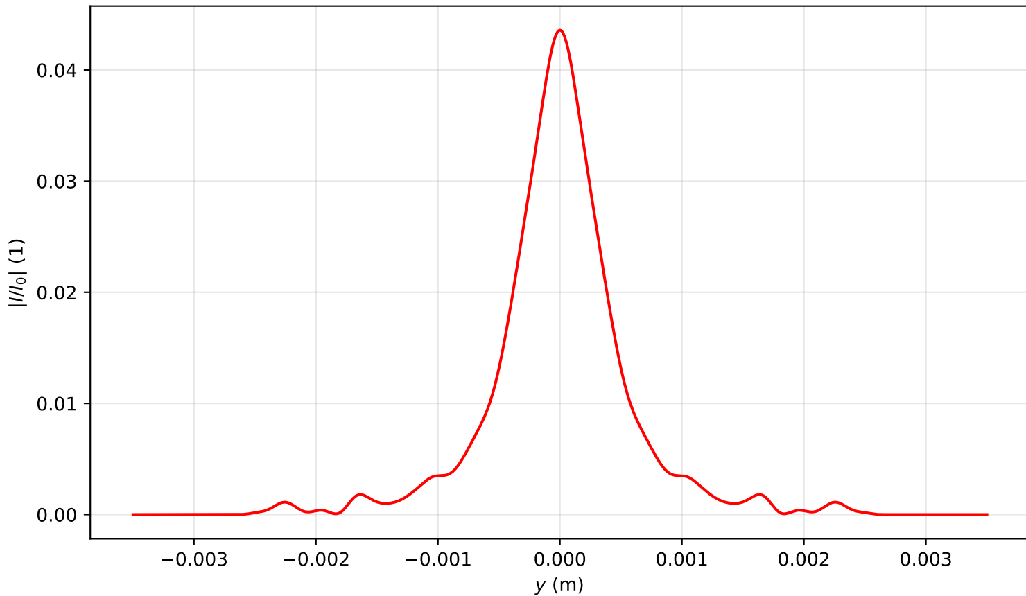
Intensity profile I(x=0, y, z=3.981)/I_0 , P_{in}=18.0P_{cr} , artificial time
