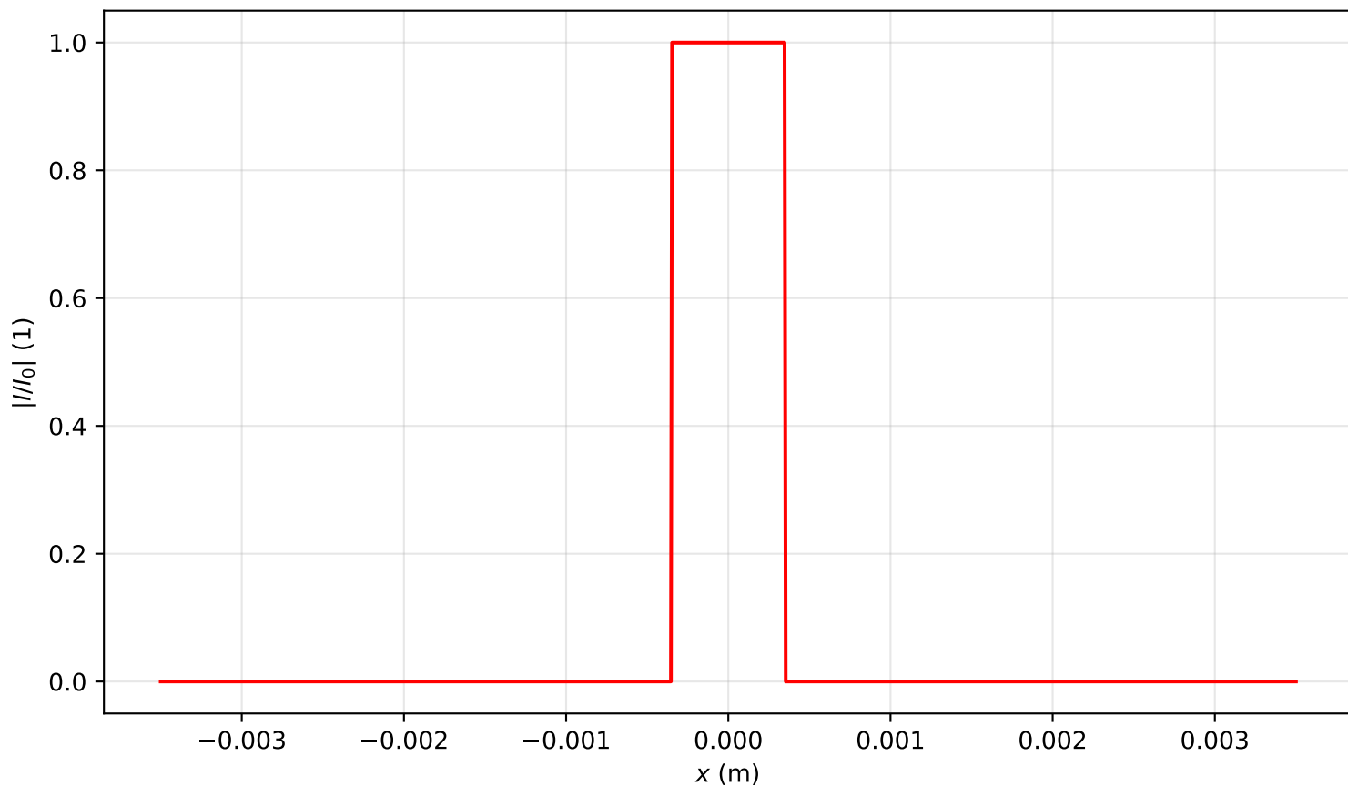
Intensity profile I(x, y = 0, z = 0.000)/I_0 , P_{in}=19.0P_{cr} , artificial time
