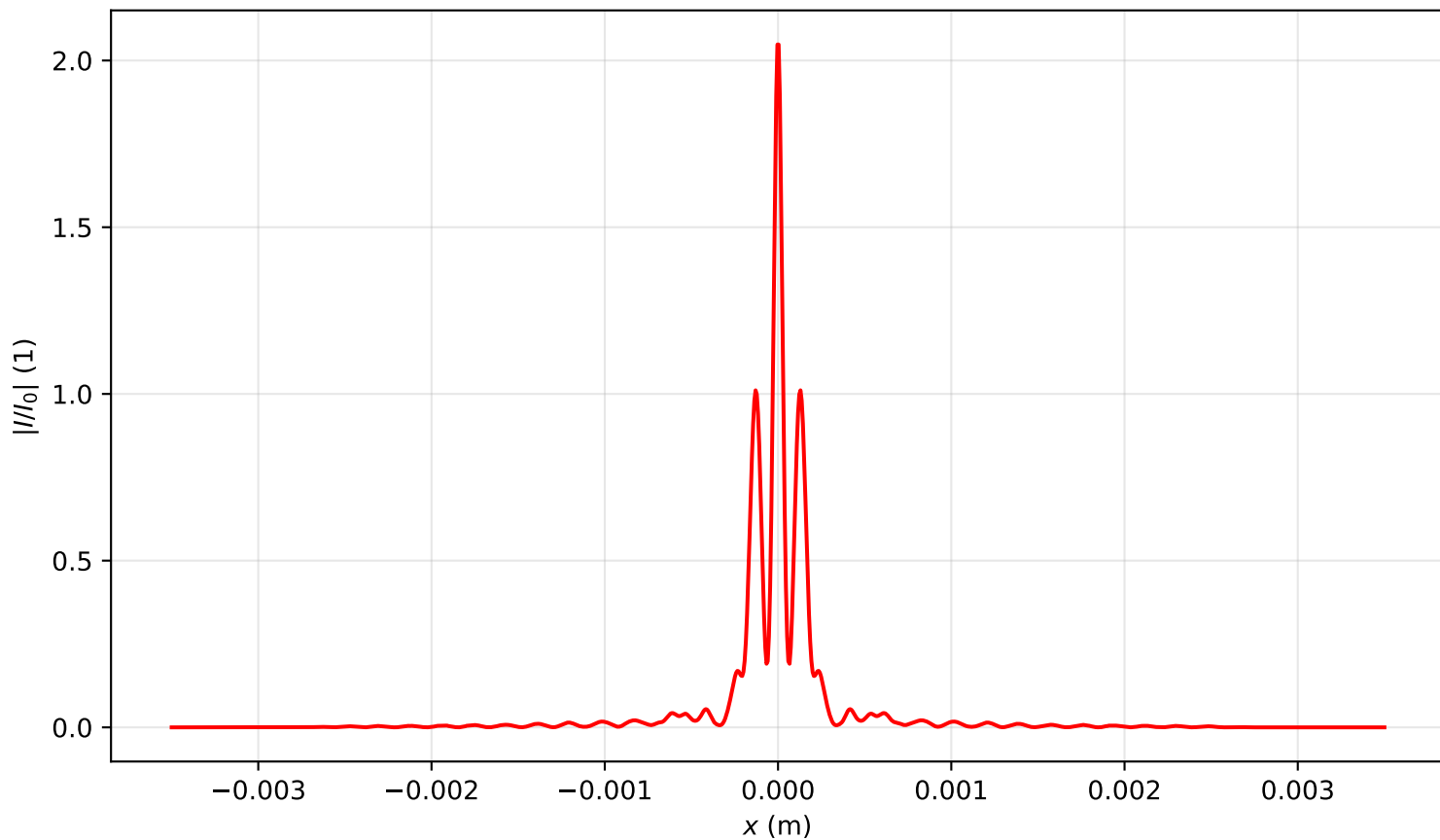
Intensity profile I(x, y = 0, z = 0.159)/I_0 , P_{in}=19.0P_{cr} , artificial time
