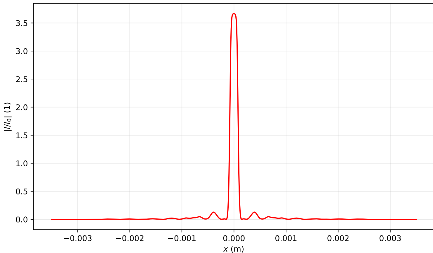
Intensity profile I(x, y = 0, z = 0.318)/I_0 , P_{in}=19.0P_{cr} , artificial time
