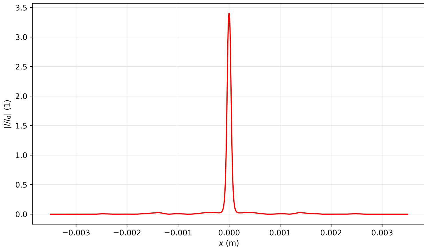
Intensity profile I(x, y = 0, z = 0.637)/I_0 , P_{in}=19.0P_{cr} , artificial time
