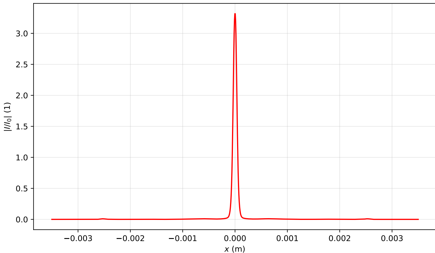
Intensity profile I(x, y = 0, z = 1.115)/I_0 , P_{in}=19.0P_{cr} , artificial time
