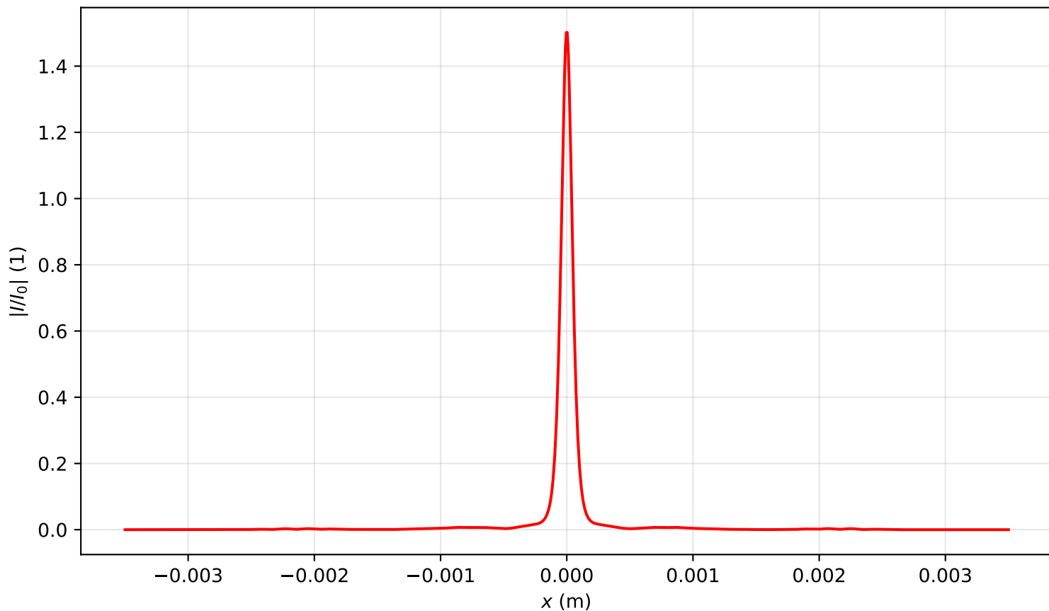
Intensity profile I(x, y = 0, z = 1.274)/I_0 , P_{in}=19.0P_{cr} , artificial time
