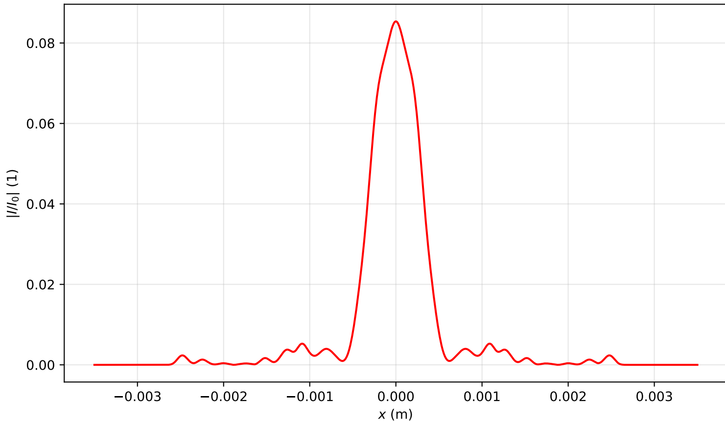
Intensity profile I(x, y = 0, z = 1.592)/I_0 , P_{in}=19.0\text{Pcr} , artificial time
