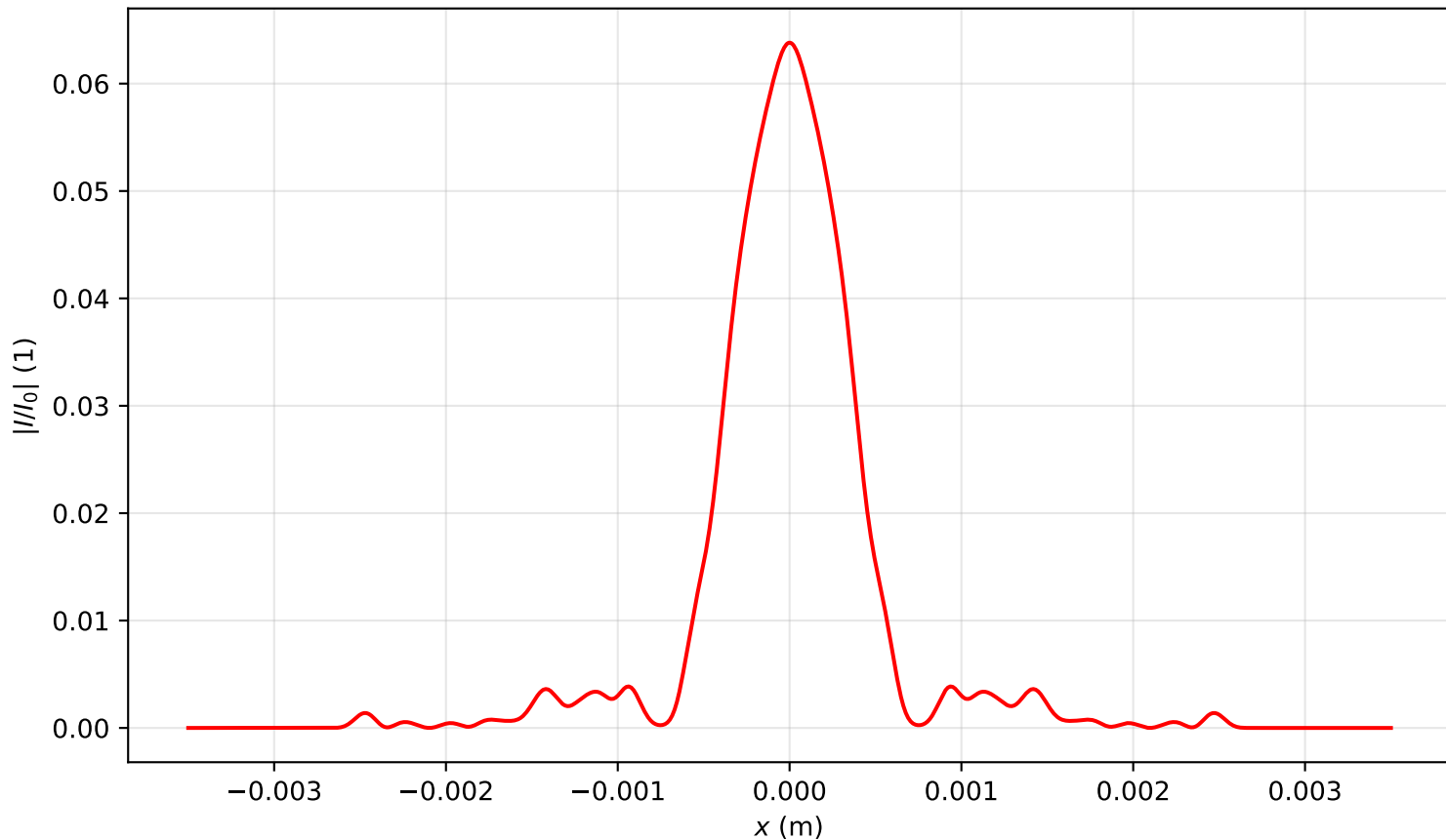
Intensity profile I(x, y = 0, z = 1.751)/I_0 , P_{in}=19.0P_{cr} , artificial time
