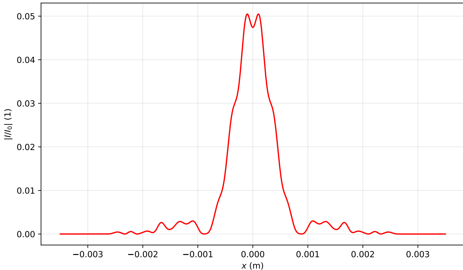
Intensity profile I(x, y = 0, z = 1.911)/I_0 , P_{in}=19.0P_{cr} , artificial time
