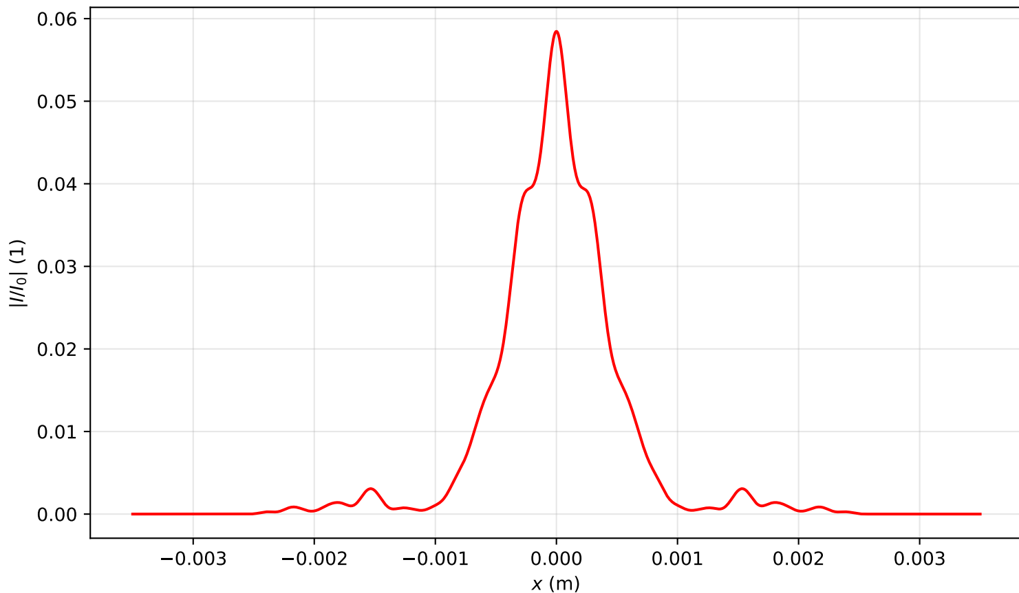
Intensity profile I(x, y = 0, z = 2.229)/I_0 , P_{in}=19.0P_{cr} , artificial time
