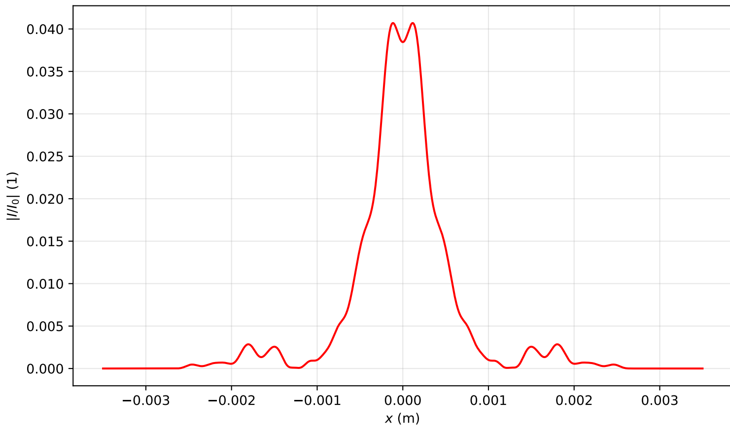
Intensity profile I(x, y = 0, z = 2.388)/I_0 , P_{in}=19.0P_{cr} , artificial time
