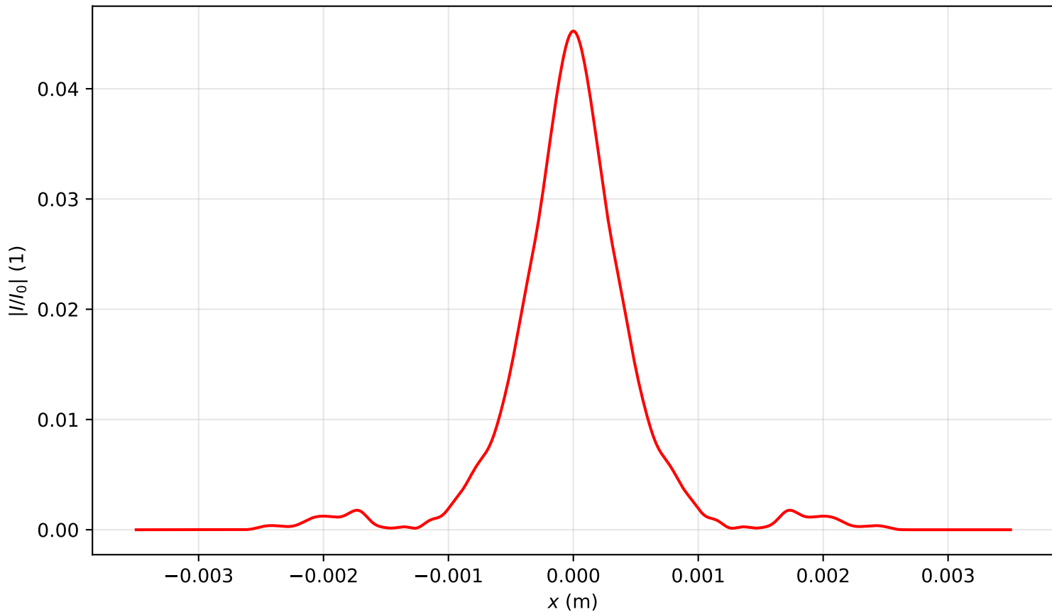
Intensity profile I(x, y = 0, z = 2.548)/I_0 , P_{in}=19.0P_{cr} , artificial time
