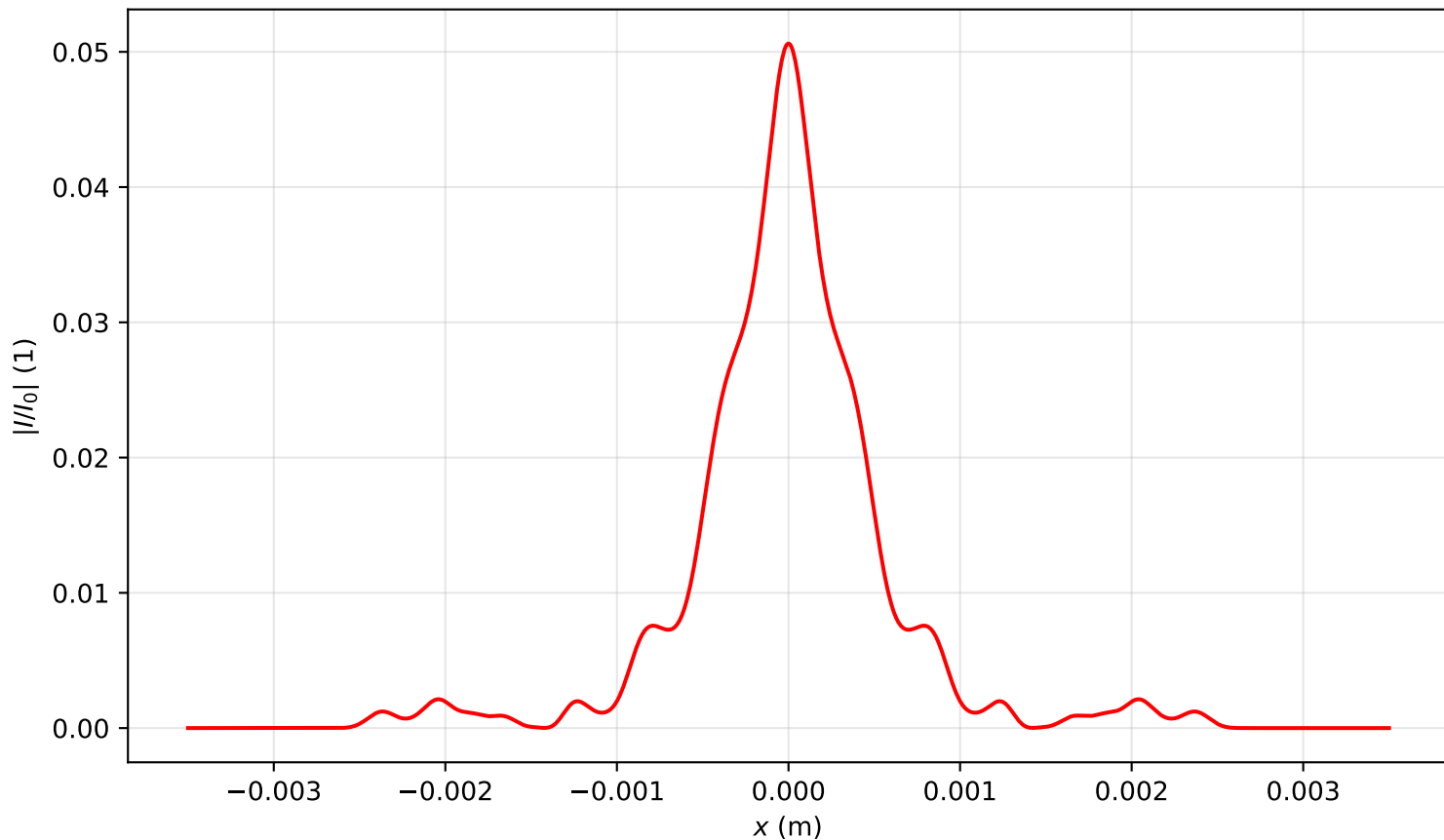
Intensity profile I(x, y = 0, z = 2.707)/I_0 , P_{in}=19.0P_{cr} , artificial time
