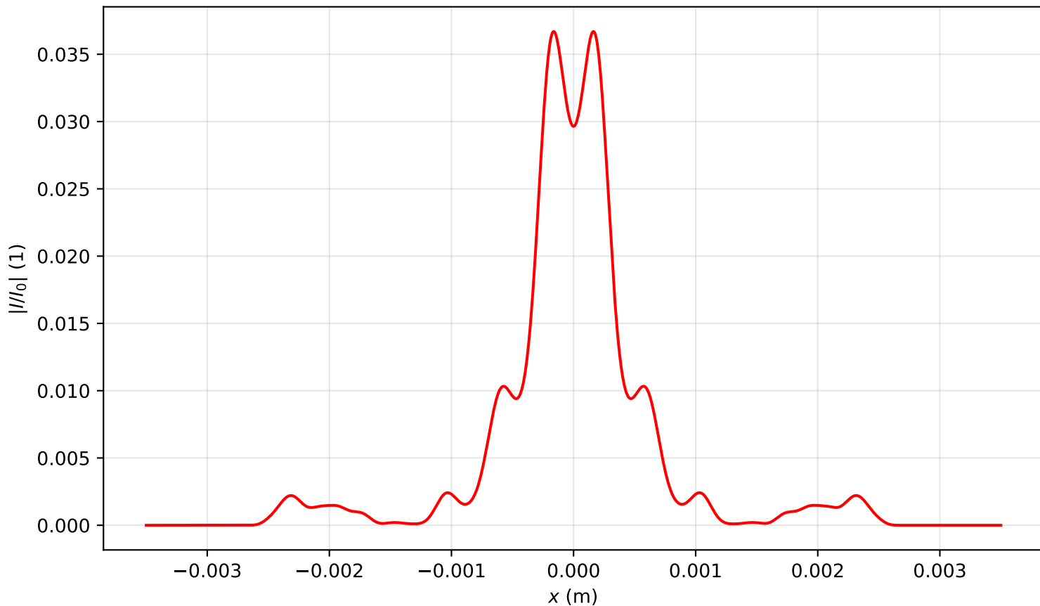
Intensity profile I(x, y = 0, z = 2.866)/I_0 , P_{in}=19.0\text{Pcr} , artificial time
