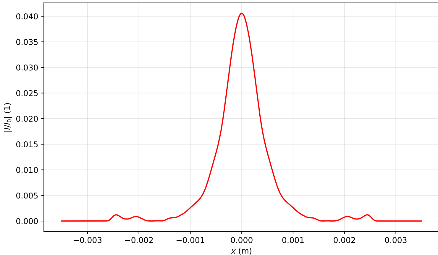
Intensity profile I(x, y = 0, z = 3.025)/I_0 , P_{in}=19.0P_{cr} , artificial time
