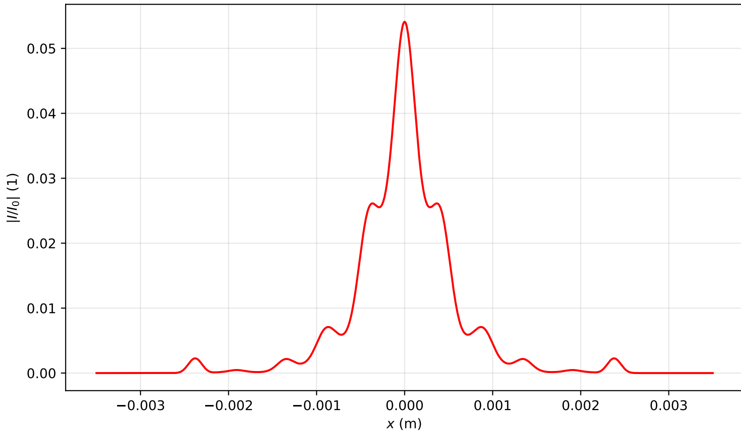
Intensity profile I(x, y = 0, z = 3.184)/I_0 , P_{in}=19.0\text{Pcr} , artificial time
