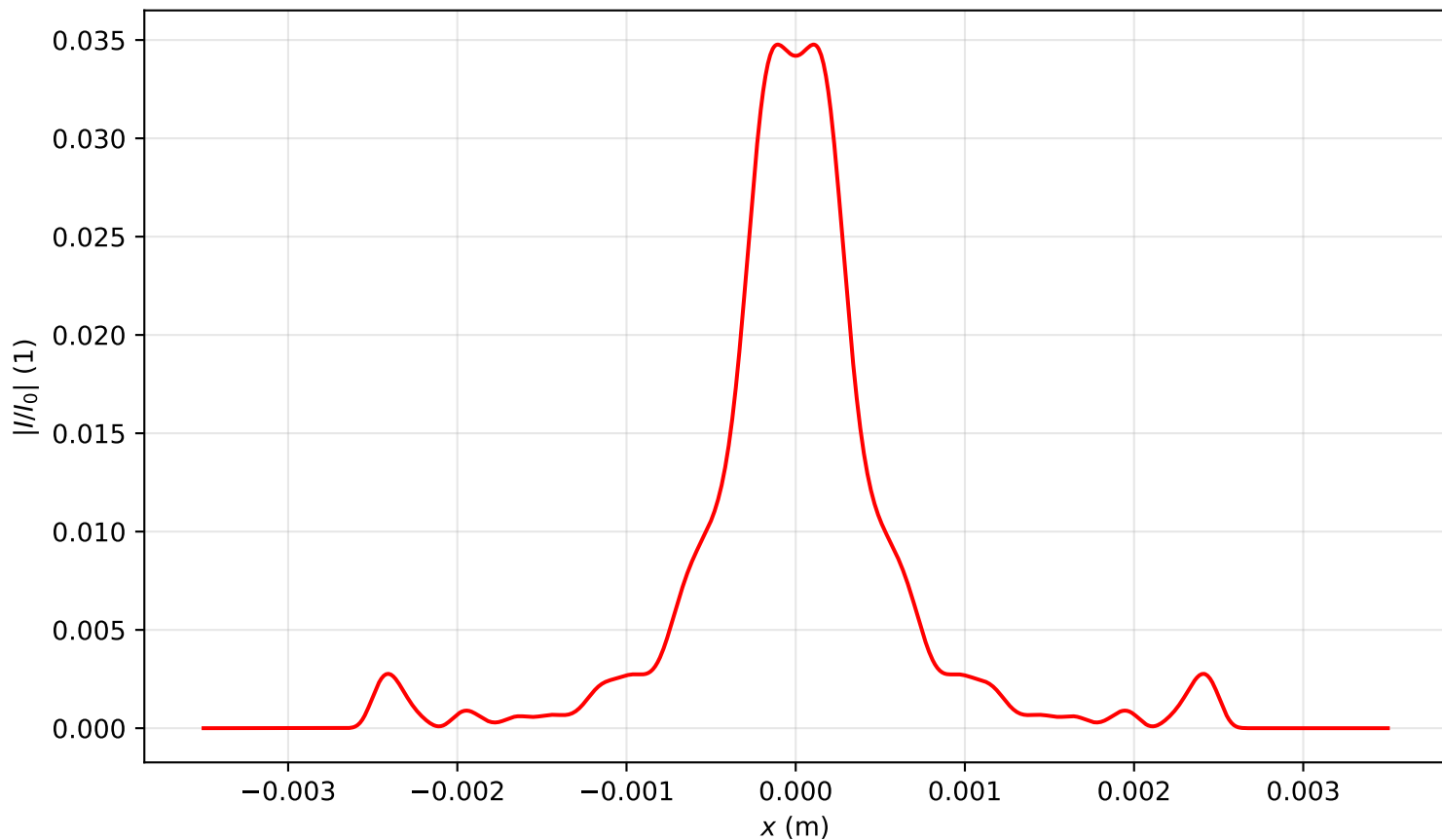
Intensity profile I(x, y = 0, z = 3.344)/I_0 , P_{in}=19.0\text{Pcr} , artificial time
