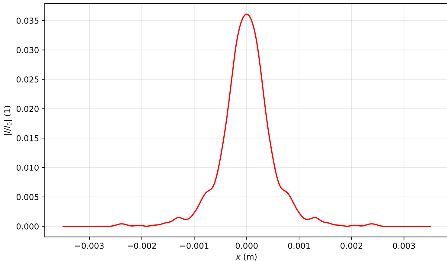
Intensity profile I(x, y = 0, z = 3.662)/I_0 , P_{in}=19.0\text{Pcr} , artificial time
