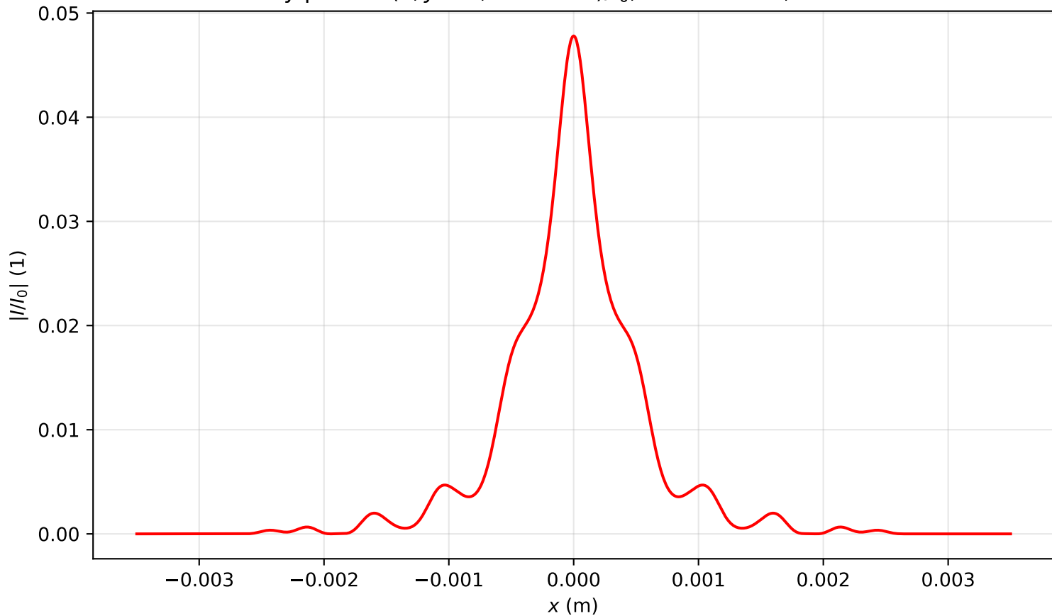
Intensity profile I(x, y = 0, z = 3.821)/I_0 , P_{in}=19.0P_{cr} , artificial time
