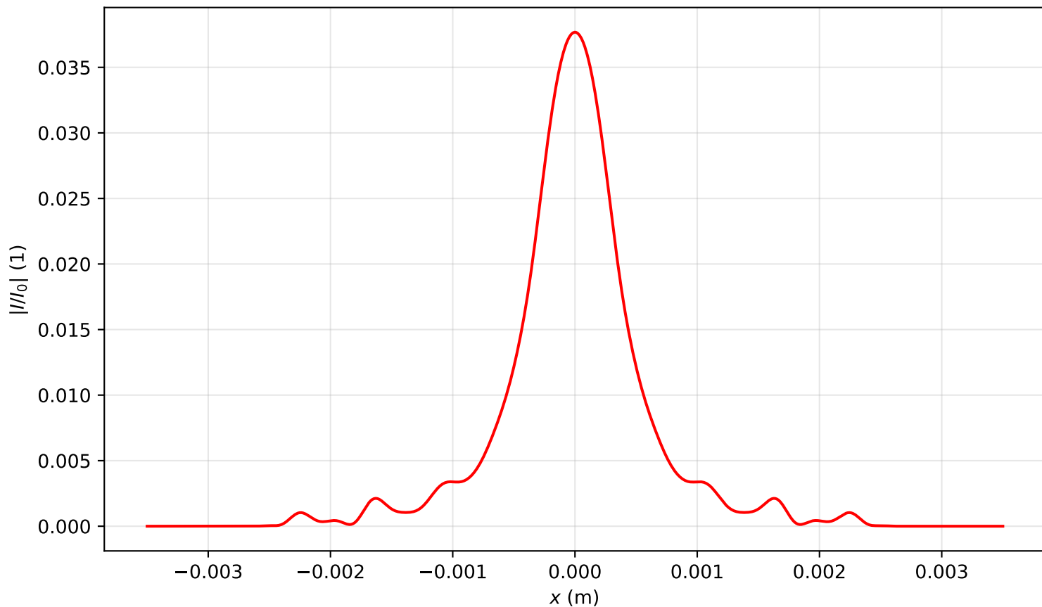
Intensity profile I(x, y = 0, z = 3.981)/I_0 , P_{in}=19.0\text{Pcr} , artificial time
