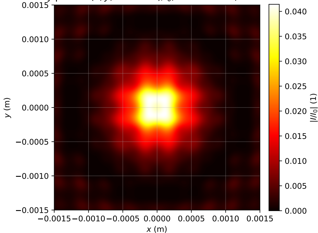
Intensity profile I(x, y, z = 2.388)/I_0 , P_{in}=19.0P_{cr} , artificial time
