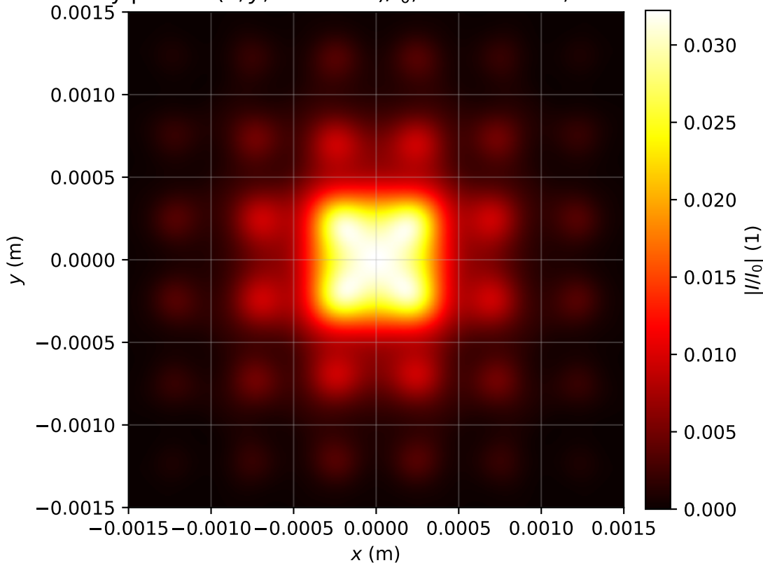
Intensity profile I(x, y, z = 3.503)/I_0 , P_{in}=19.0P_{cr} , artificial time
