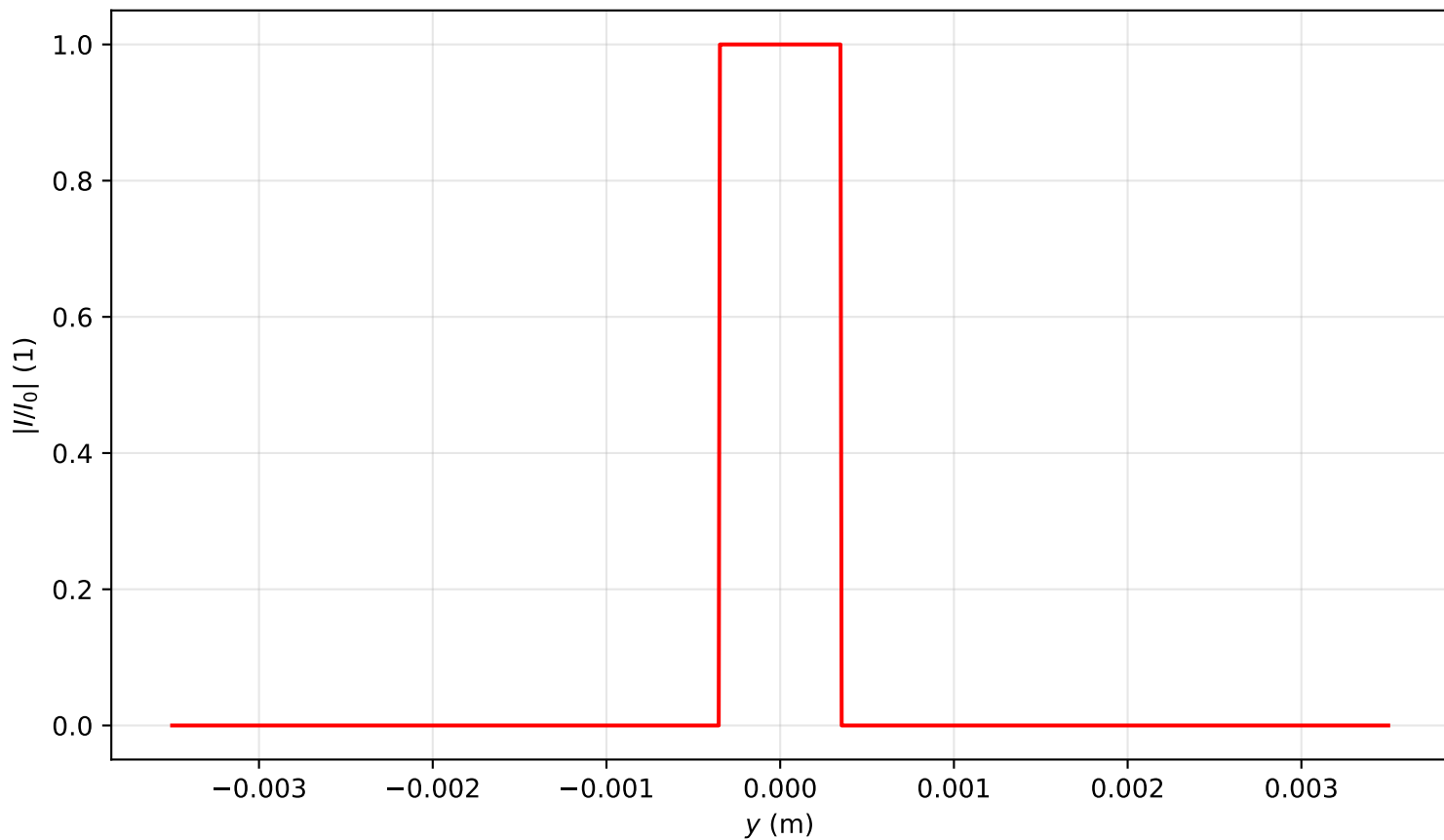
Intensity profile I(x=0, y, z=0.000)/I_0 , P_{in}=19.0\text{Pcr} , artificial time
