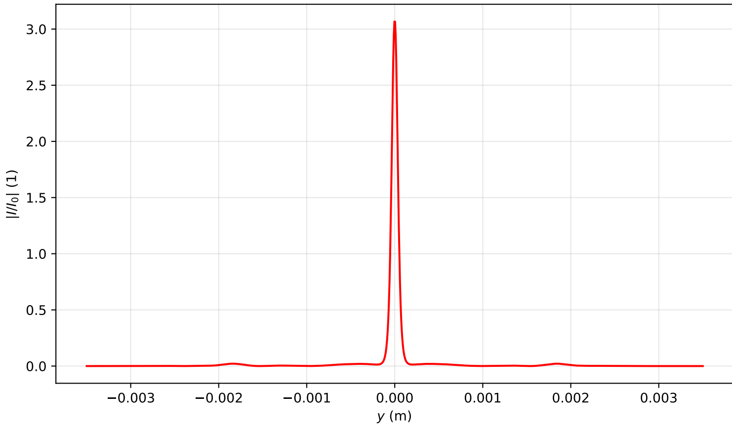
Intensity profile I(x=0, y, z=0.796)/I_0 , P_{in}=19.0P_{cr} , artificial time
