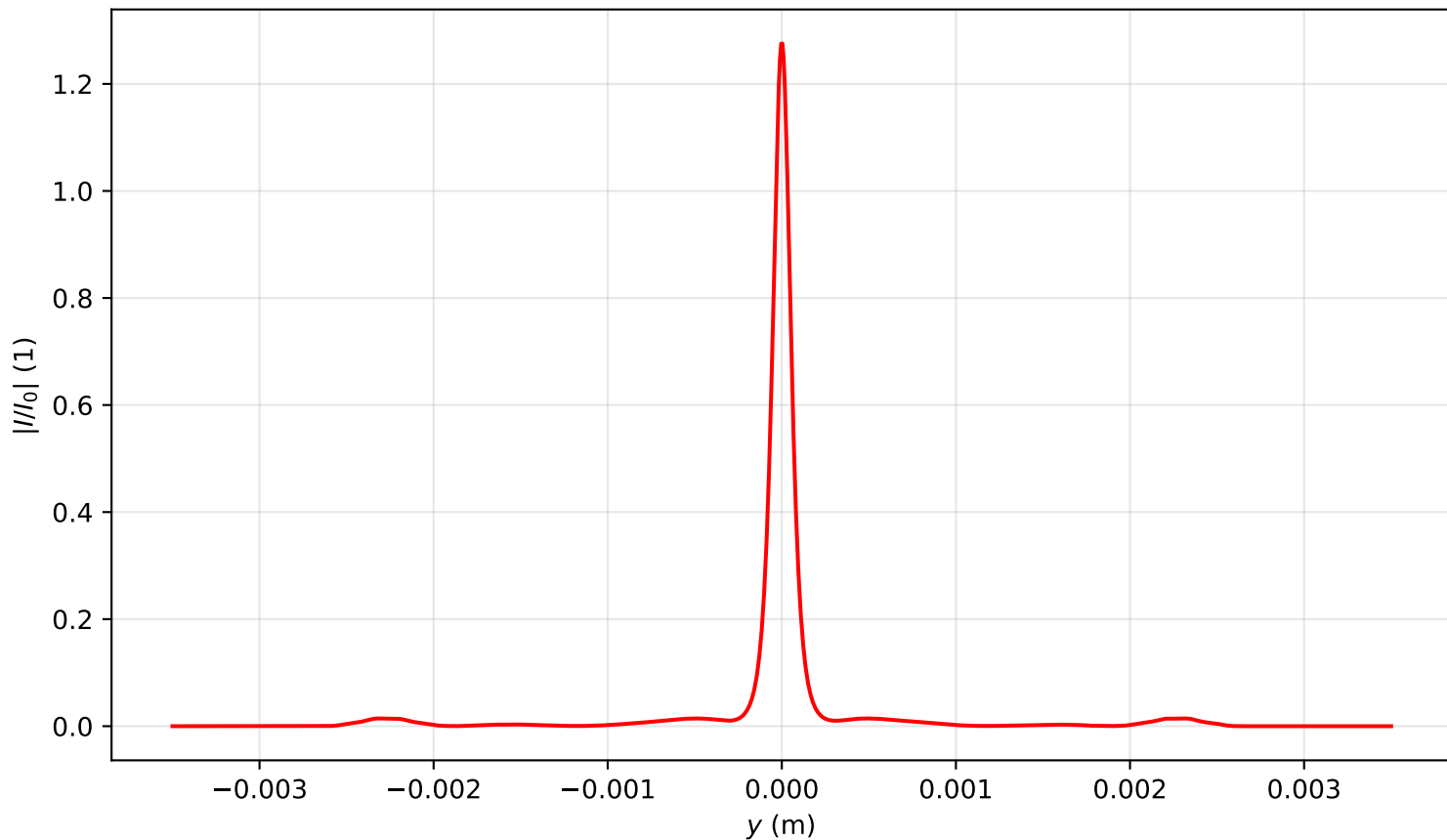
Intensity profile I(x=0, y, z=0.955)/I_0 , P_{in}=19.0P_{cr} , artificial time
