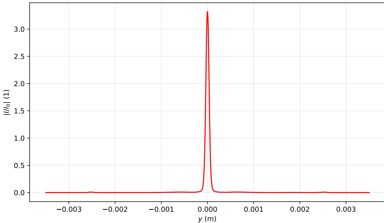
Intensity profile I(x=0, y, z=1.115)/I_0 , P_{in}=19.0P_{cr} , artificial time
