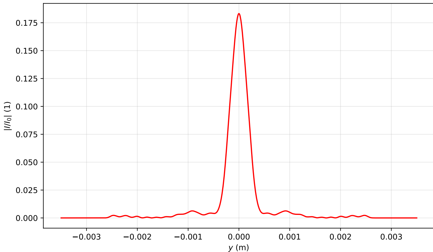
Intensity profile I(x=0, y, z=1.433)/I_0 , P_{in}=19.0P_{cr} , artificial time
