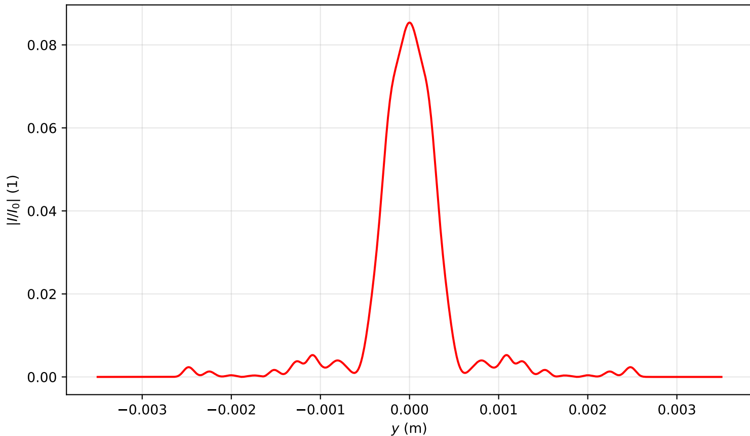
Intensity profile I(x = 0, y, z = 1.592)/I_0 , P_{in}=19.0\text{Pcr} , artificial time
