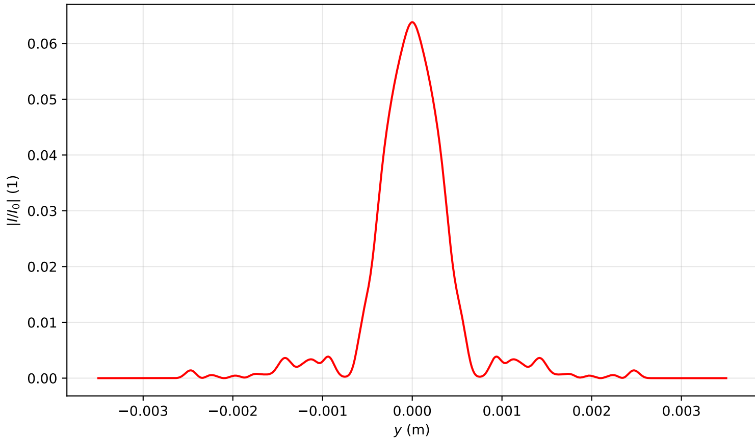
Intensity profile I(x = 0, y, z = 1.751)/I_0 , P_{in}=19.0\text{Pcr} , artificial time
